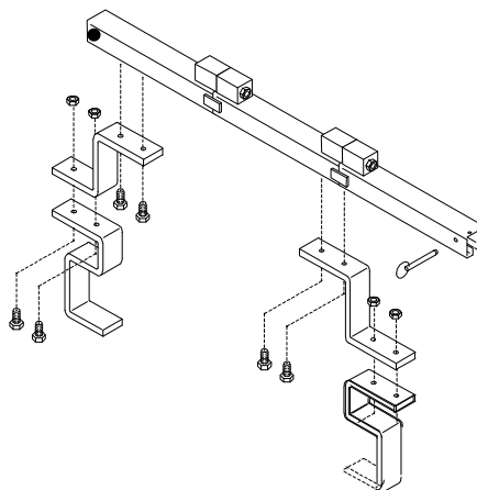
HOIST TOP RAIL PARTS WITH ELEVATING BRACKETS
