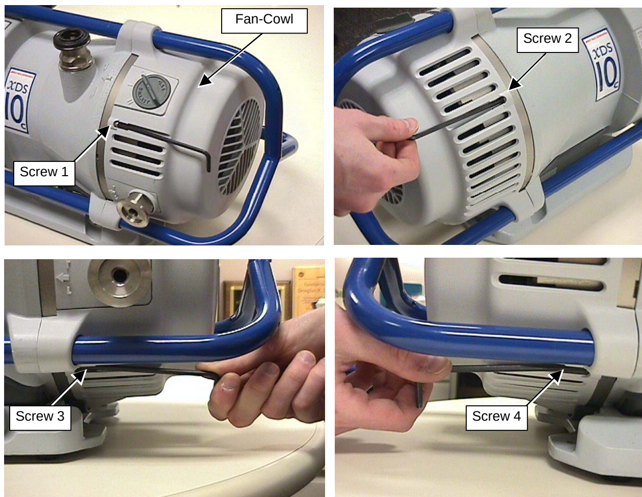
VACUUM PUMP CAP SCREWS ILLUSTRATION 9-12
