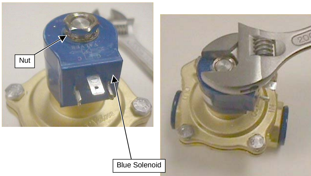
REPLACING AND SECURING BLUE SOLENOID ILLUSTRATION 9-43
